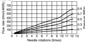
PJNC 8-04 Control flow 10-04 12-04
