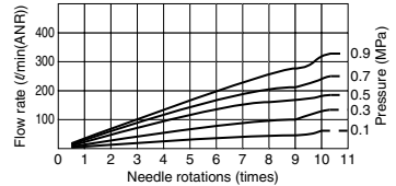
PJNC 6-03 Control flow 8-03 10-03 12-03
