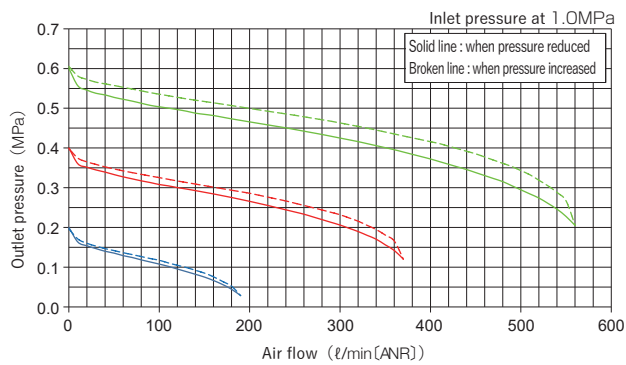
RVCP6-02, RVCMP6-02
