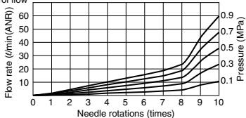
Control flow
