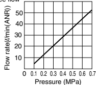
Free flow
