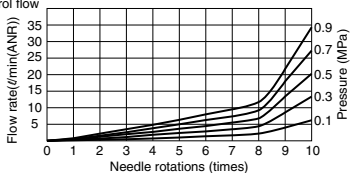
Control flow
