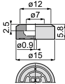
VP15F Weight : 1.1g[1.7g]
