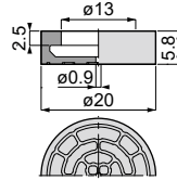
VP20F Weight : 1.4g[2.3g]
