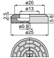
VP25F Weight : 2.6g[4.1g]
