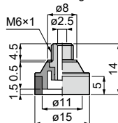
VP15S [5] - M6 [9] Weight : 2.1g[2.3g]
