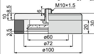
VP100S [5] - M10 [9] Weight : 272g[300g]
