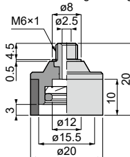
VP35S [5] - M6 [9] Weight : 35g[40g]
