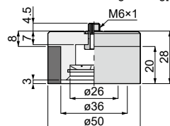
VP50S [5] - M6 [9] Weight : 76g[83g]
