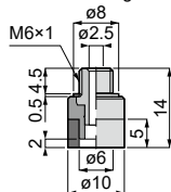
VP10S [5] - M6 [9] Weight : 1.9g[1.9g]
