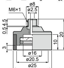
VP50S [5] - M6 [9] Weight : 76g[83g]
