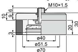
VP70S [5] - M10 [9] Weight : 142g[156g]
